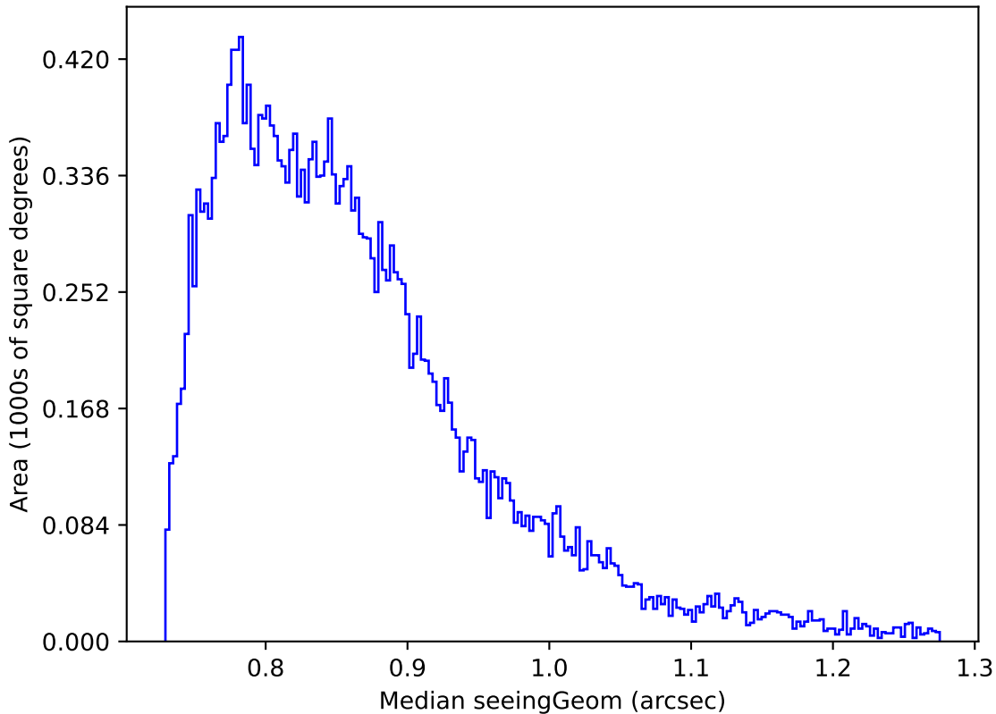
too_elab_r16_d2_giz_v3.4_10yrs Yr 1 all bands: Median seeingGeom
