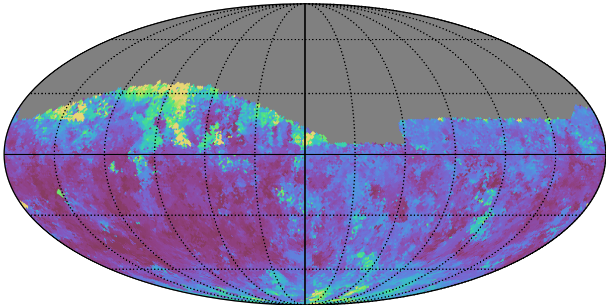
too_elab_r16_d2_giz_v3.4_10yrs Yr 1 z band: Median seeingEff
