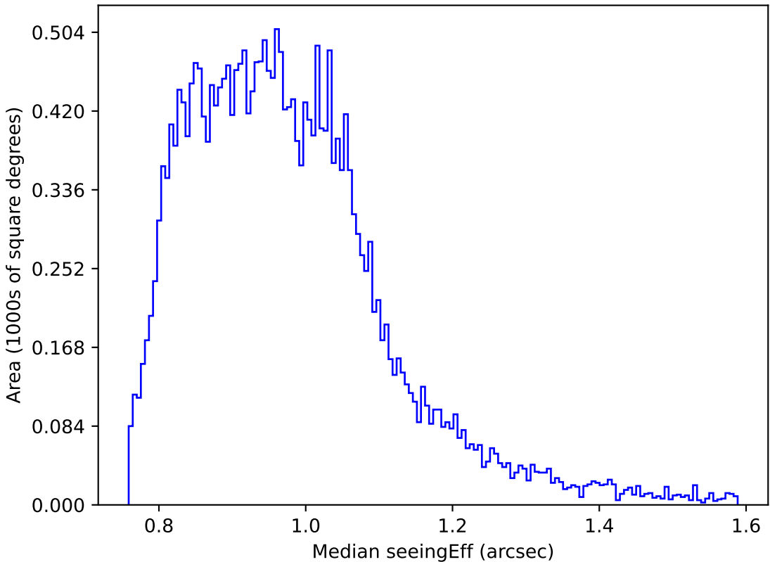
too_elab_r16_d2_giz_v3.4_10yrs Yr 1 z band: Median seeingEff
