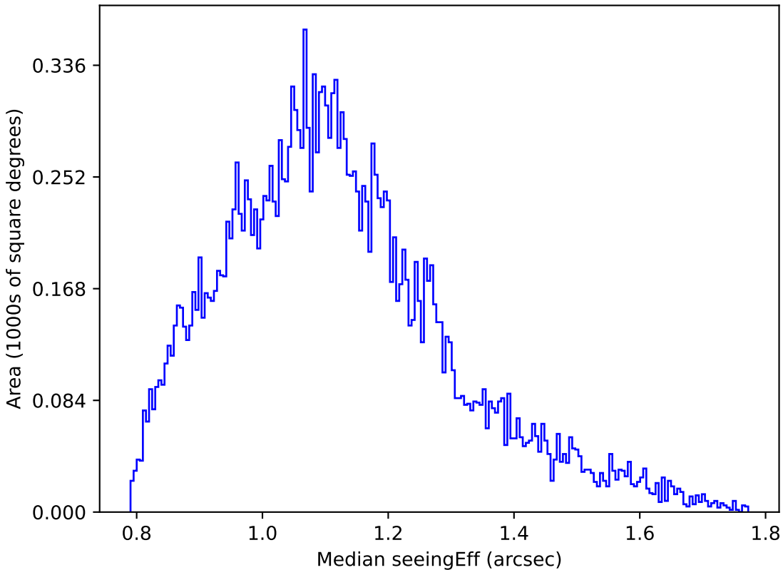
too_elab_r16_d2_giz_v3.4_10yrs Yr 1 u band: Median seeingEff
