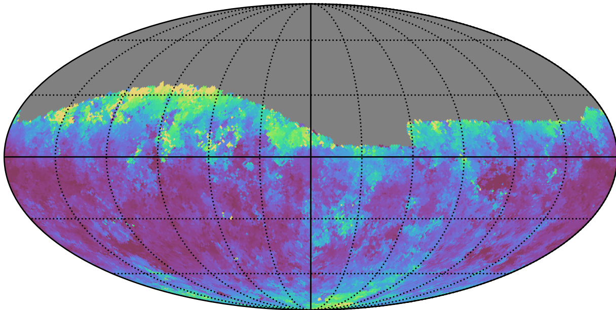
too_elab_r16_d2_giz_v3.4_10yrs Yr 1 i band: Median seeingEff
