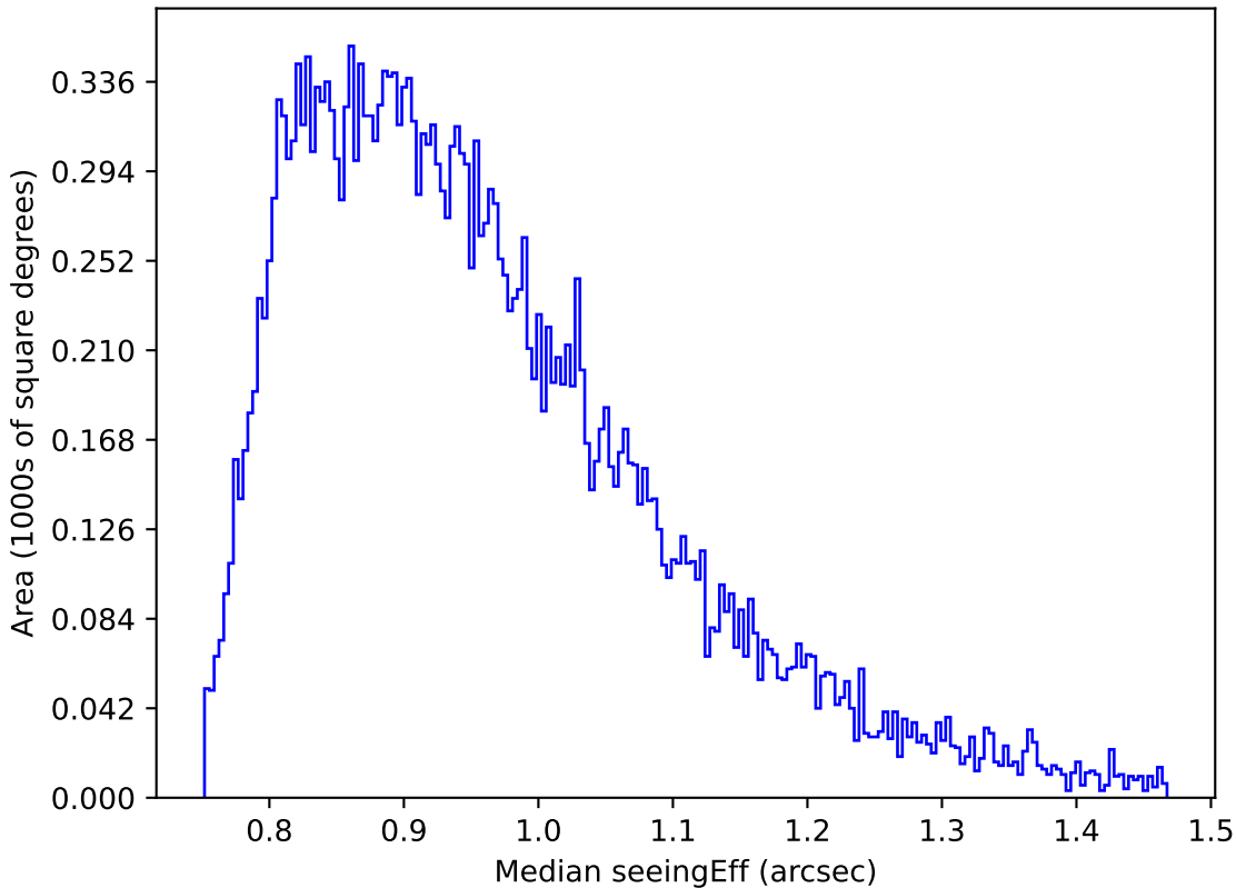
too_elab_r16_d2_giz_v3.4_10yrs Yr 1 i band: Median seeingEff
