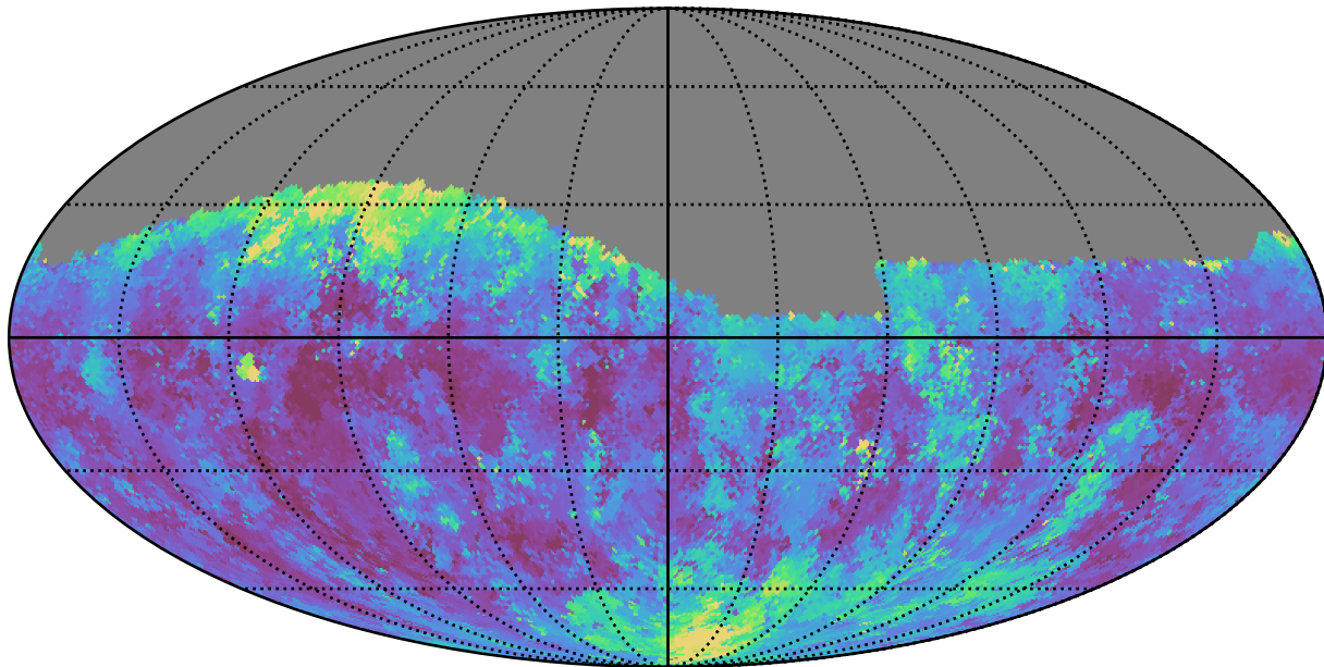
too_elab_r16_d2_giz_v3.4_10yrs Yr 1 g band: Median seeingEff
