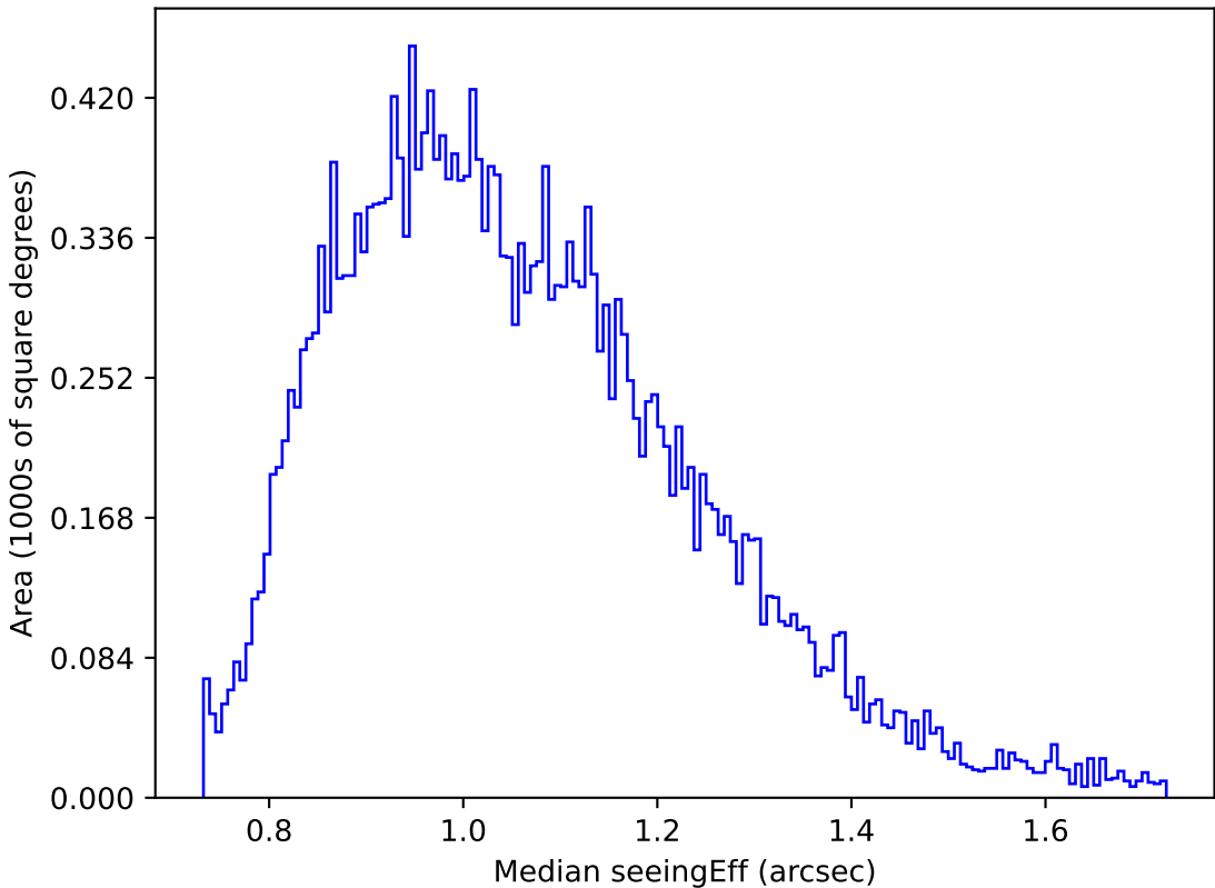
too_elab_r16_d2_giz_v3.4_10yrs Yr 1 g band: Median seeingEff
