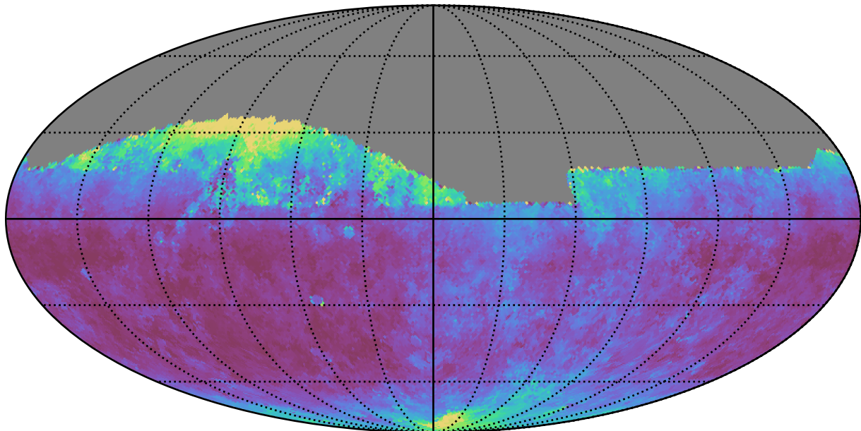
too_elab_r16_d2_giz_v3.4_10yrs Yr 1 all bands: Median seeingEff
