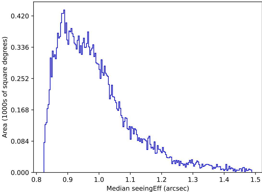
too_elab_r16_d2_giz_v3.4_10yrs Yr 1 all bands: Median seeingEff
