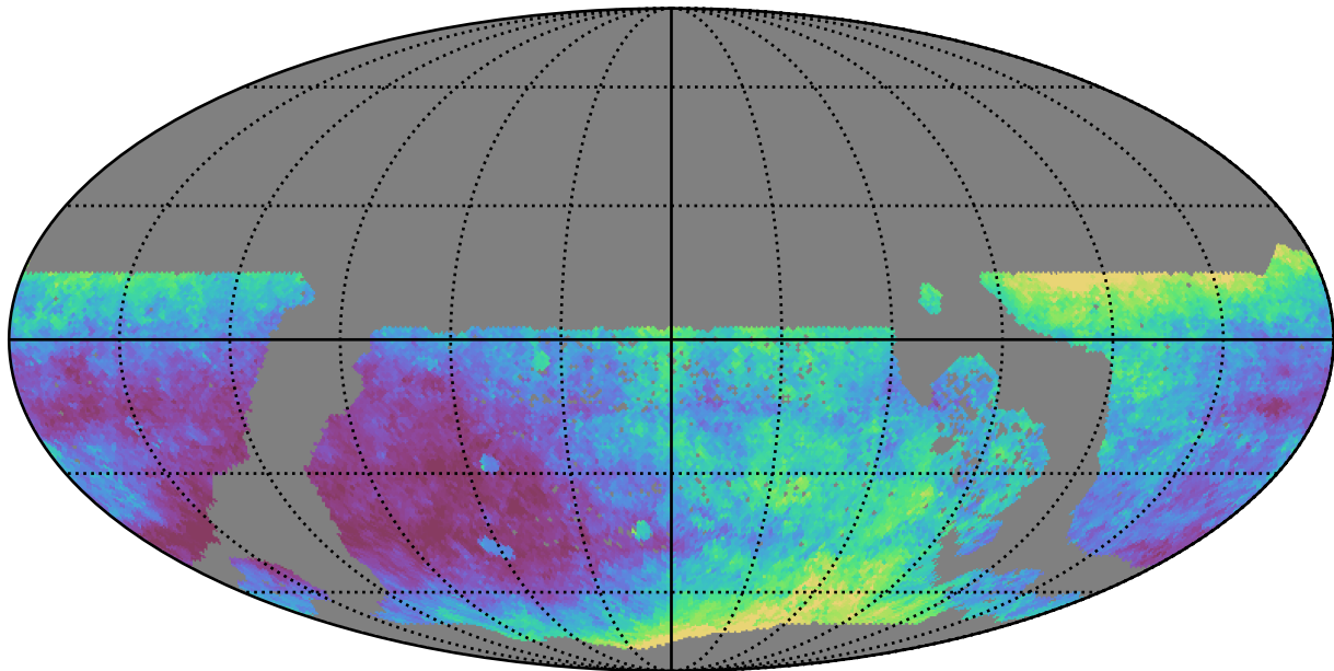
too_elab_r16_d2_giz_v3.4_10yrs WFD z band: Median seeingEff
