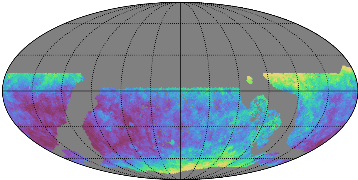
too_elab_r16_d2_giz_v3.4_10yrs WFD y band: Median seeingEff
