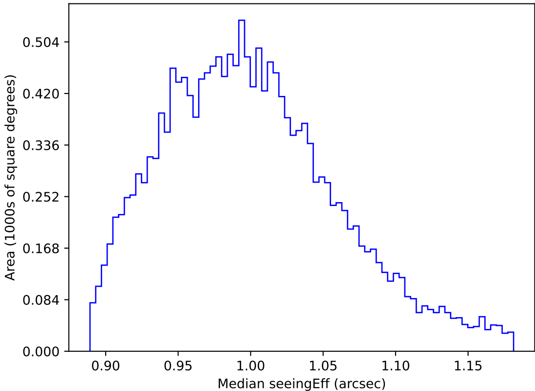
too_elab_r16_d2_giz_v3.4_10yrs WFD y band: Median seeingEff
