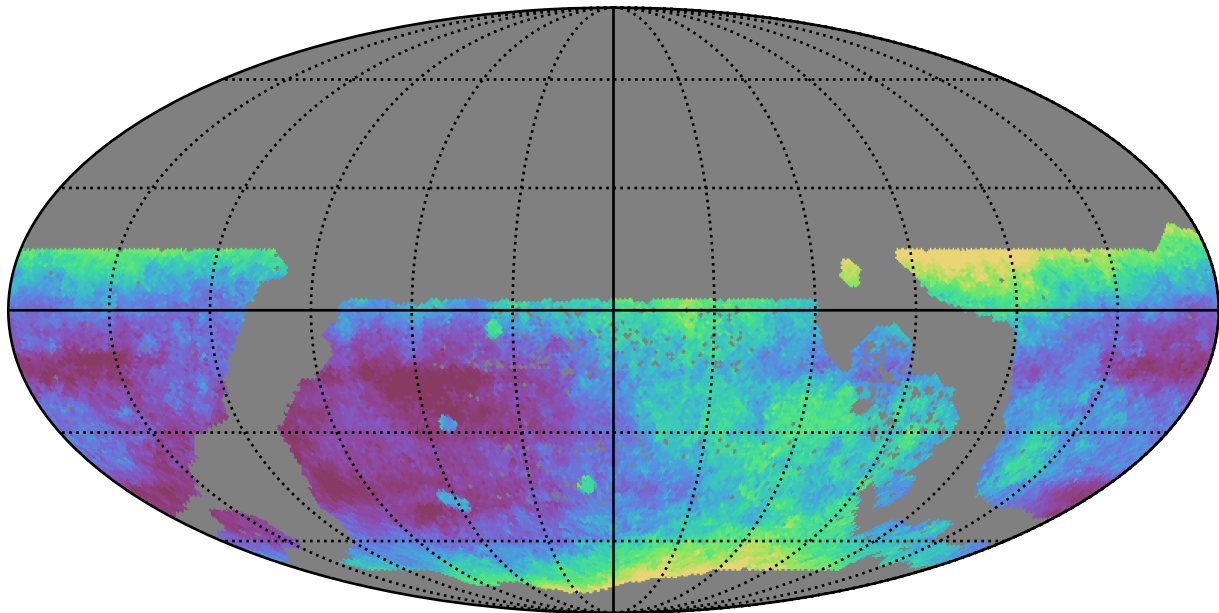
too_elab_r16_d2_giz_v3.4_10yrs WFD r band: Median seeingEff
