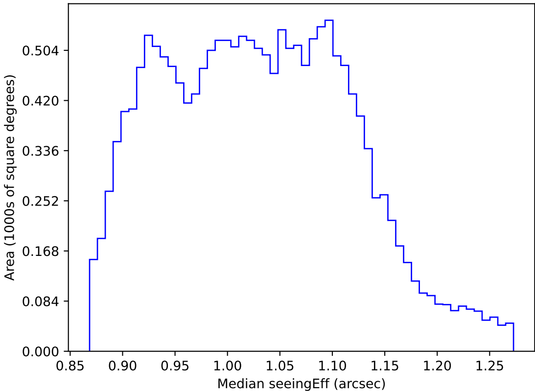
too_elab_r16_d2_giz_v3.4_10yrs WFD r band: Median seeingEff
