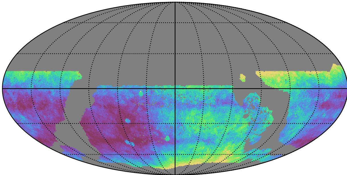
too_elab_r16_d2_giz_v3.4_10yrs WFD i band: Median seeingEff
