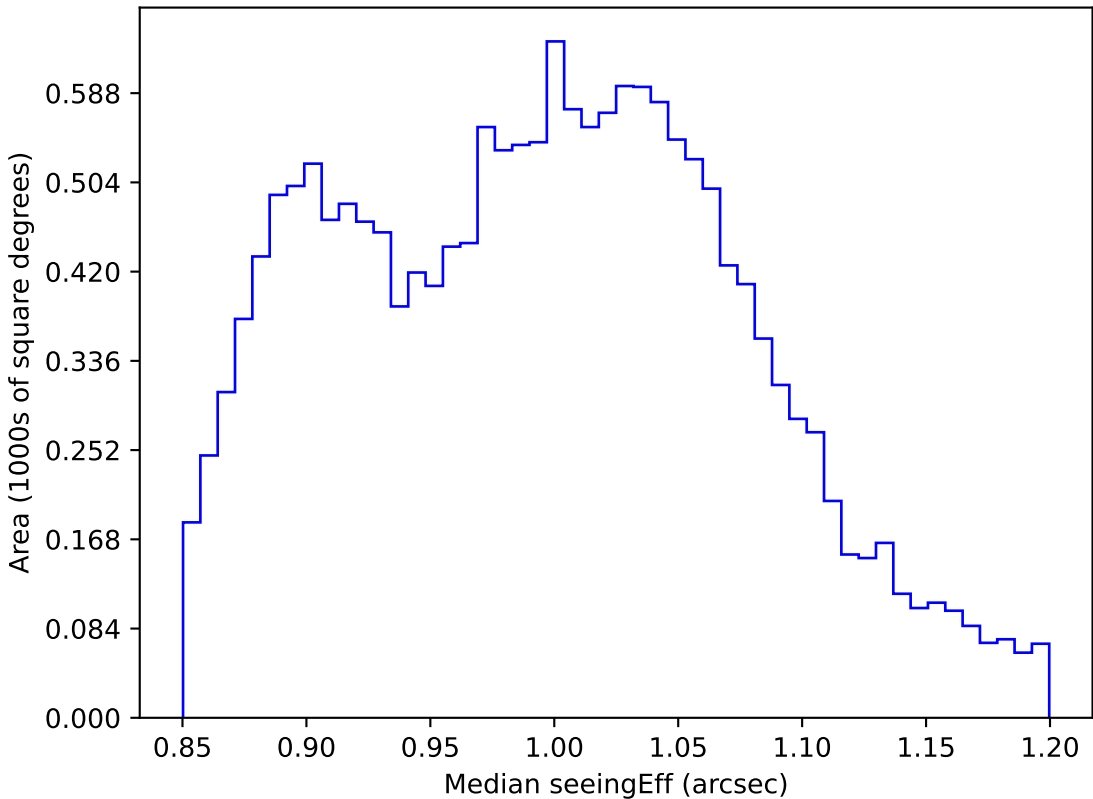
too_elab_r16_d2_giz_v3.4_10yrs WFD i band: Median seeingEff
