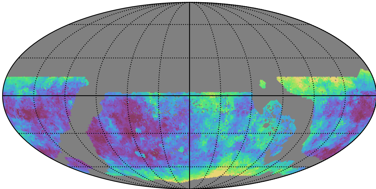
too_elab_r16_d2_giz_v3.4_10yrs WFD g band: Median seeingEff
