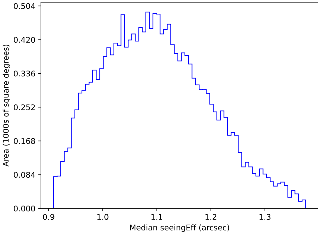
too_elab_r16_d2_giz_v3.4_10yrs WFD g band: Median seeingEff
