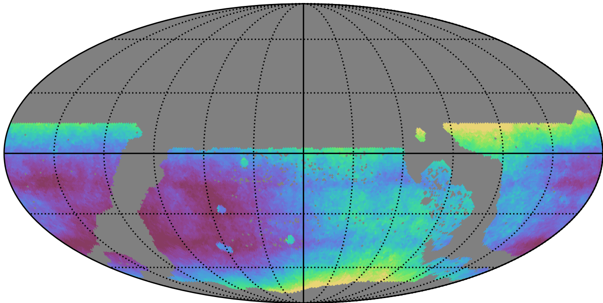
too_elab_r16_d2_giz_v3.4_10yrs WFD all bands: Median seeingEff
