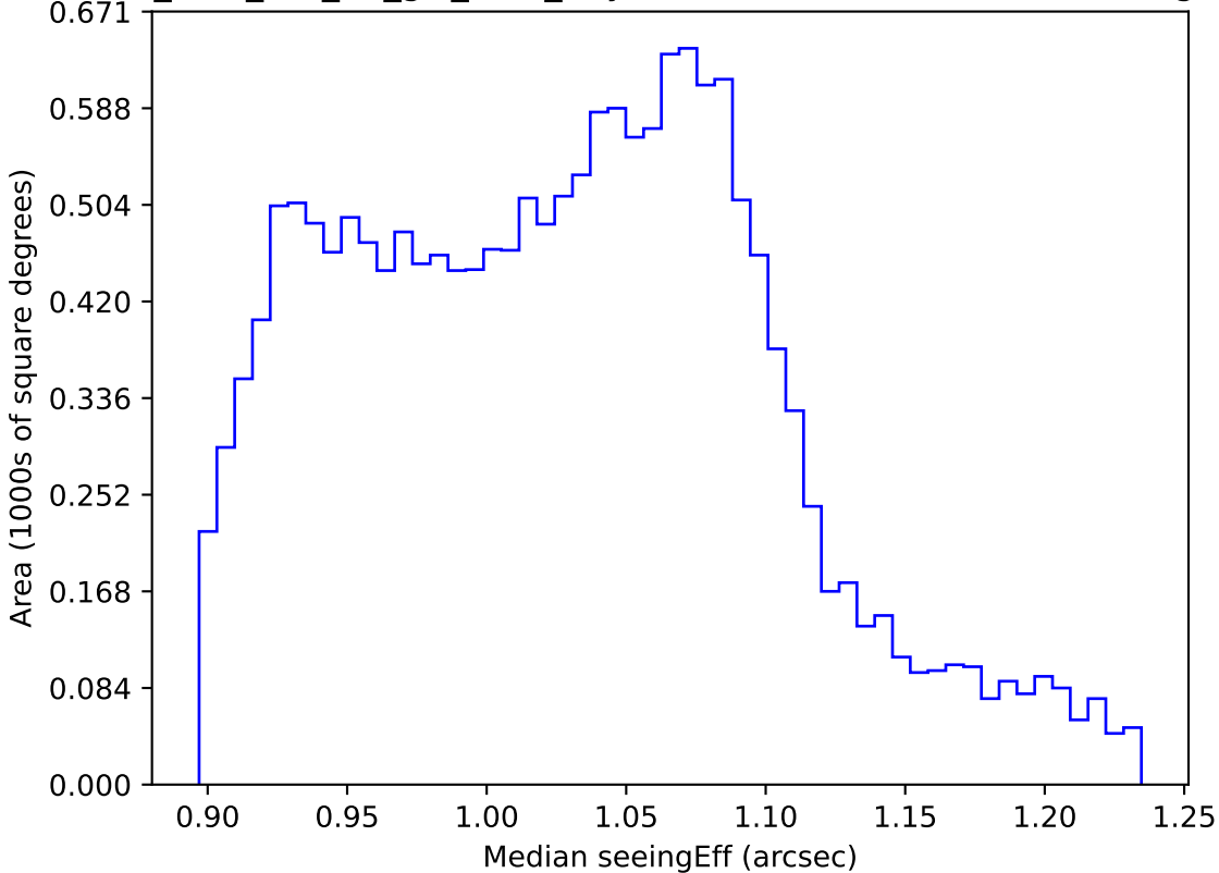
too_elab_r16_d2_giz_v3.4_10yrs WFD all bands: Median seeingEff
