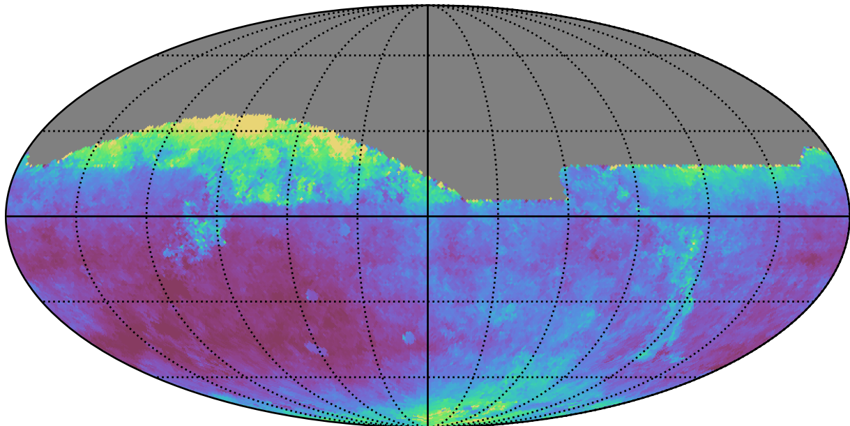
too_elab_r16_d2_giz_v3.4_10yrs All sky z band: Median seeingEff
