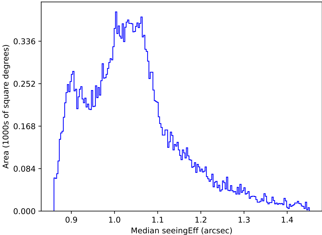
too_elab_r16_d2_giz_v3.4_10yrs All sky z band: Median seeingEff
