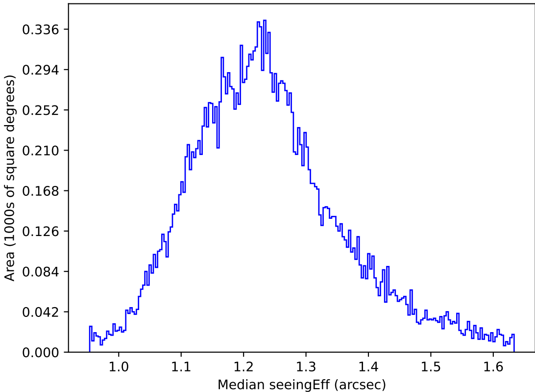
too_elab_r16_d2_giz_v3.4_10yrs All sky u band: Median seeingEff
