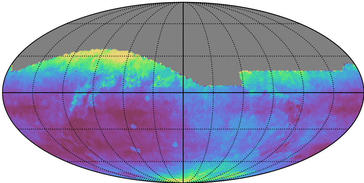
too_elab_r16_d2_giz_v3.4_10yrs All sky r band: Median seeingEff
