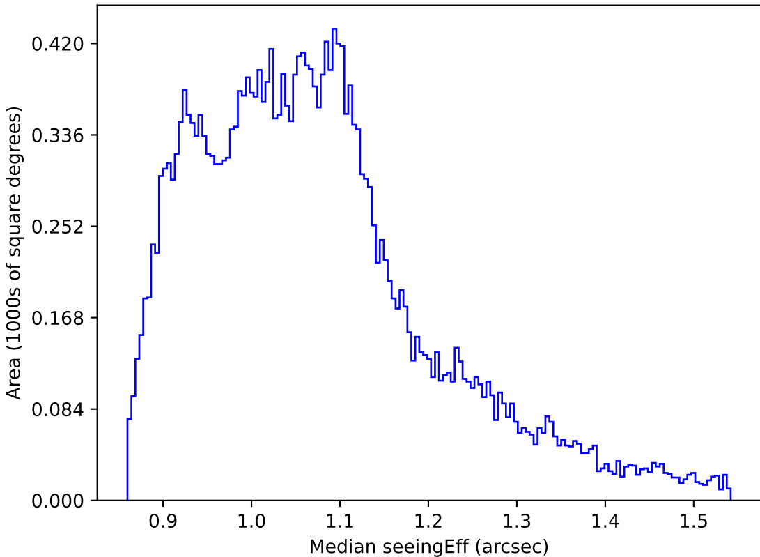
too_elab_r16_d2_giz_v3.4_10yrs All sky r band: Median seeingEff
