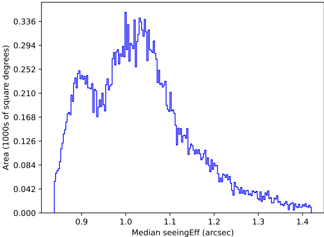
too_elab_r16_d2_giz_v3.4_10yrs All sky i band: Median seeingEff
