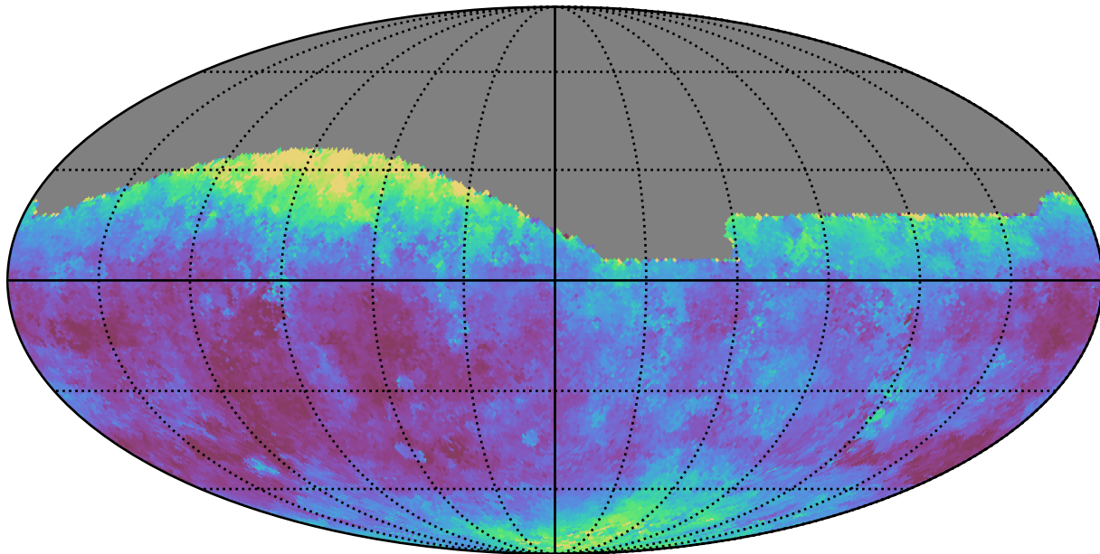
too_elab_r16_d2_giz_v3.4_10yrs All sky g band: Median seeingEff
