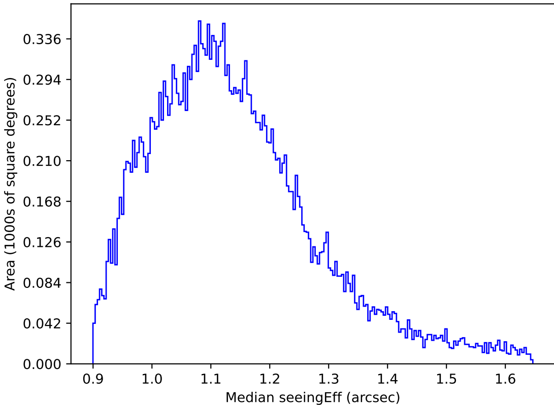
too_elab_r16_d2_giz_v3.4_10yrs All sky g band: Median seeingEff
