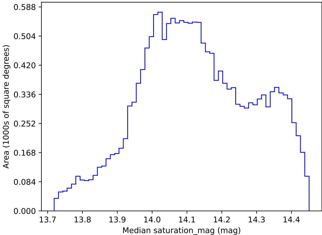
too_elab_r16_d2_giz_v3.4_10yrs WFD z band: Median saturation_mag
