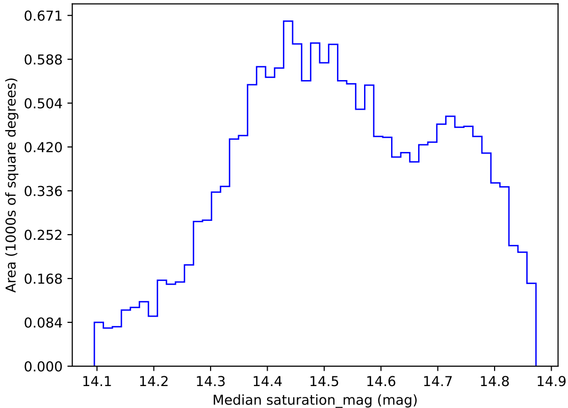
too_elab_r16_d2_giz_v3.4_10yrs WFD i band: Median saturation_mag
