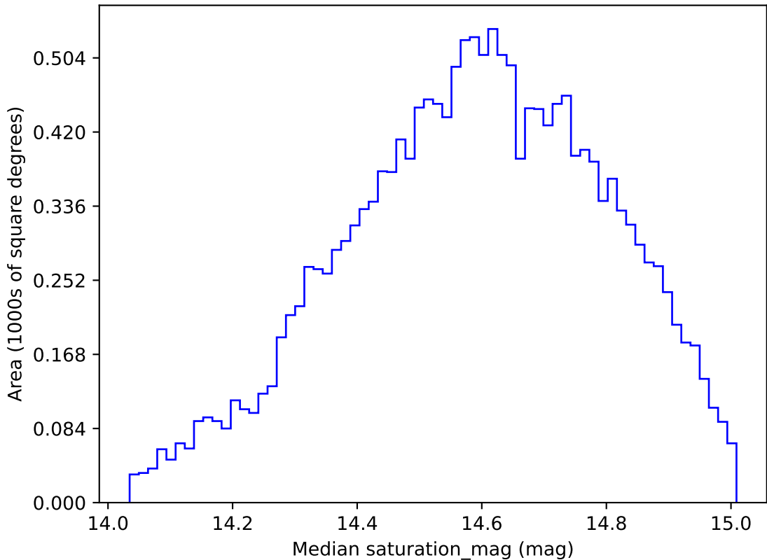
too_elab_r16_d2_giz_v3.4_10yrs WFD g band: Median saturation_mag
