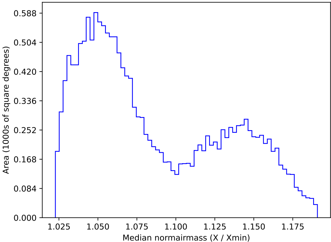
too_elab_r16_d2_giz_v3.4_10yrs WFD z band: Median normairmass
