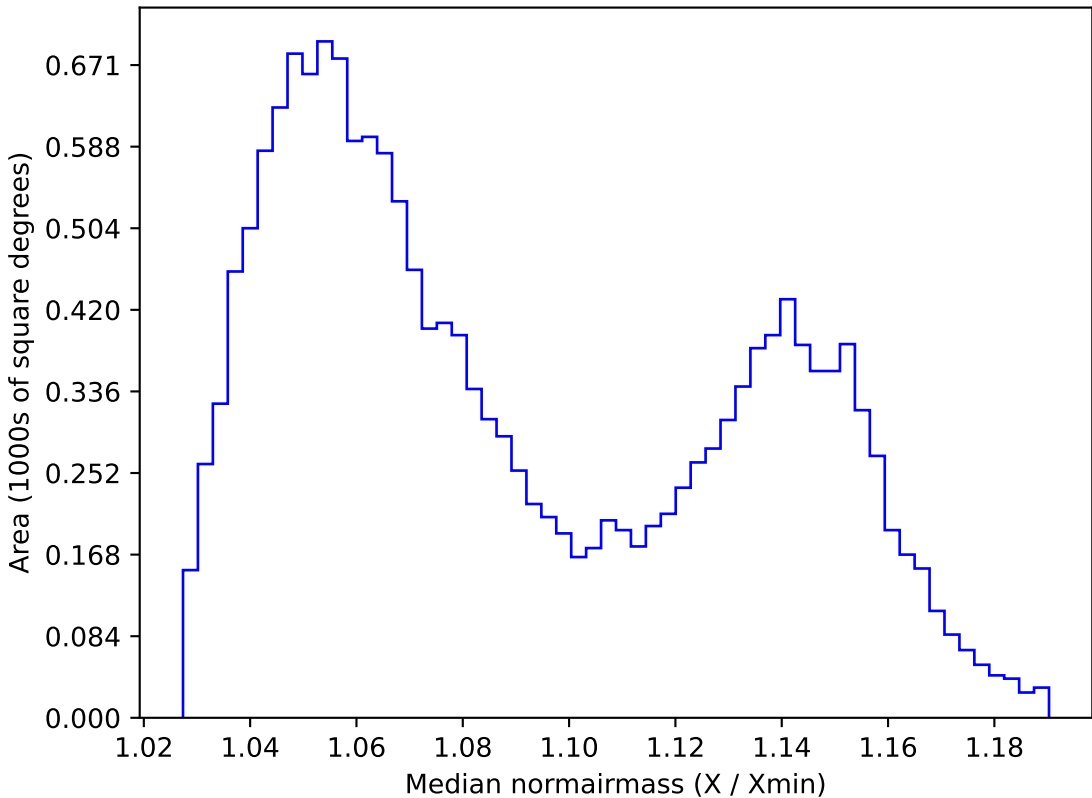
too_elab_r16_d2_giz_v3.4_10yrs WFD y band: Median normairmass
