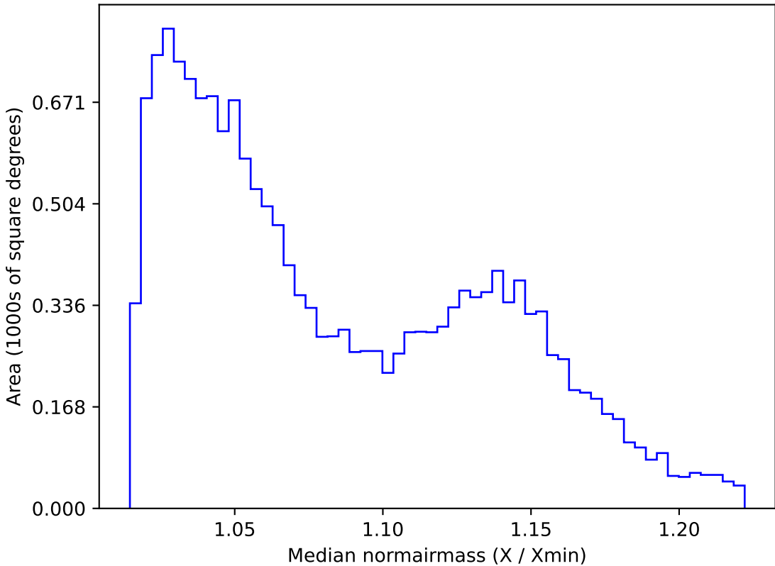
too_elab_r16_d2_giz_v3.4_10yrs WFD g band: Median normairmass
