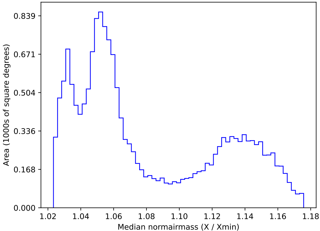
too_elab_r16_d2_giz_v3.4_10yrs WFD all bands: Median normairmass
