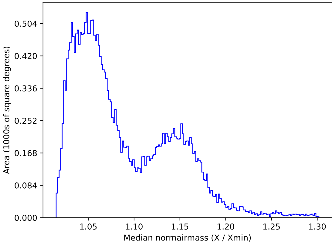
too_elab_r16_d2_giz_v3.4_10yrs All sky z band: Median normairmass
