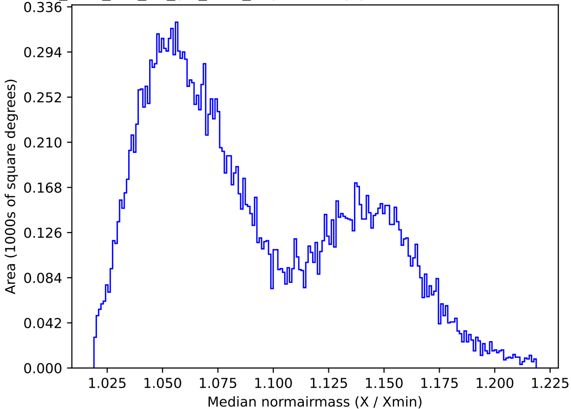
too_elab_r16_d2_giz_v3.4_10yrs All sky y band: Median normairmass
