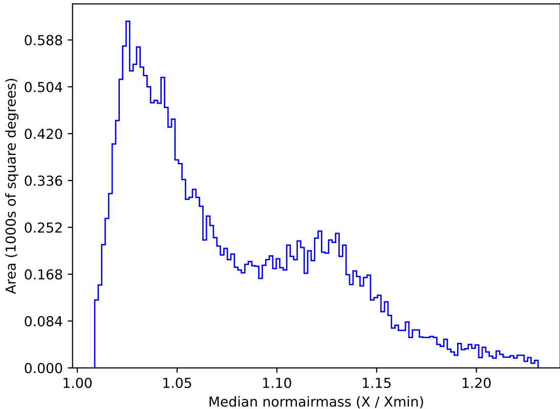
too_elab_r16_d2_giz_v3.4_10yrs All sky u band: Median normairmass
