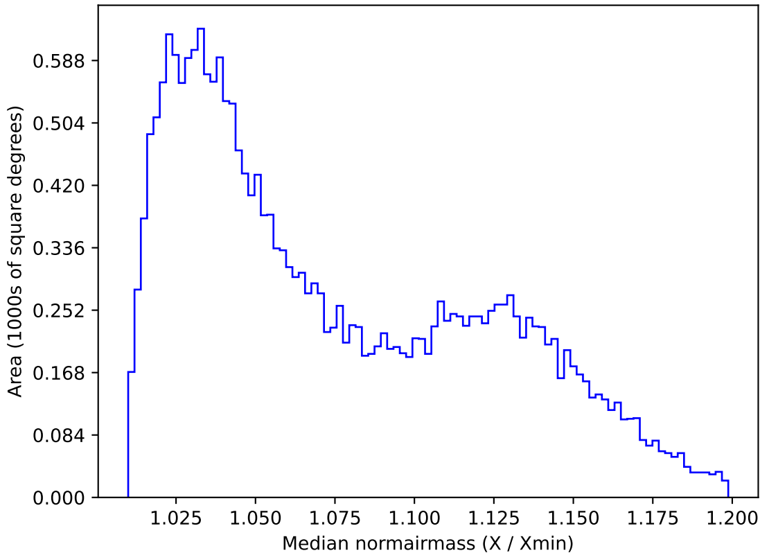
too_elab_r16_d2_giz_v3.4_10yrs All sky u band: Median normairmass
