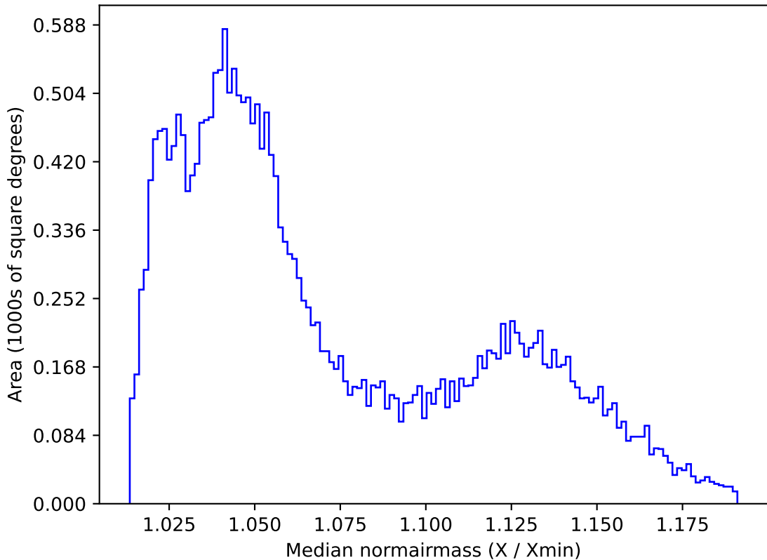
too_elab_r16_d2_giz_v3.4_10yrs All sky r band: Median normairmass
