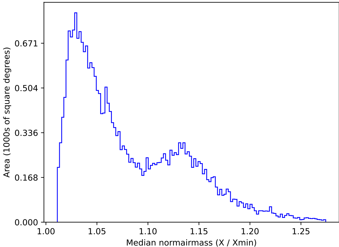
too_elab_r16_d2_giz_v3.4_10yrs All sky g band: Median normairmass
