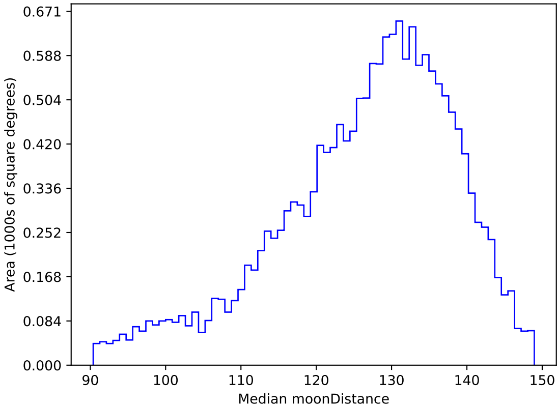
too_elab_r16_d2_giz_v3.4_10yrs WFD u band: Median moonDistance
