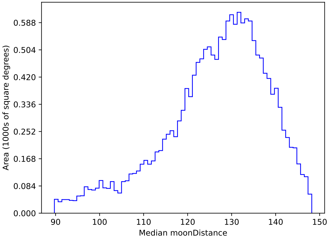
too_elab_r16_d2_giz_v3.4_10yrs WFD u band: Median moonDistance
