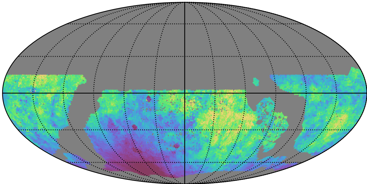
too_elab_r16_d2_giz_v3.4_10yrs WFD r band: Median moonDistance
