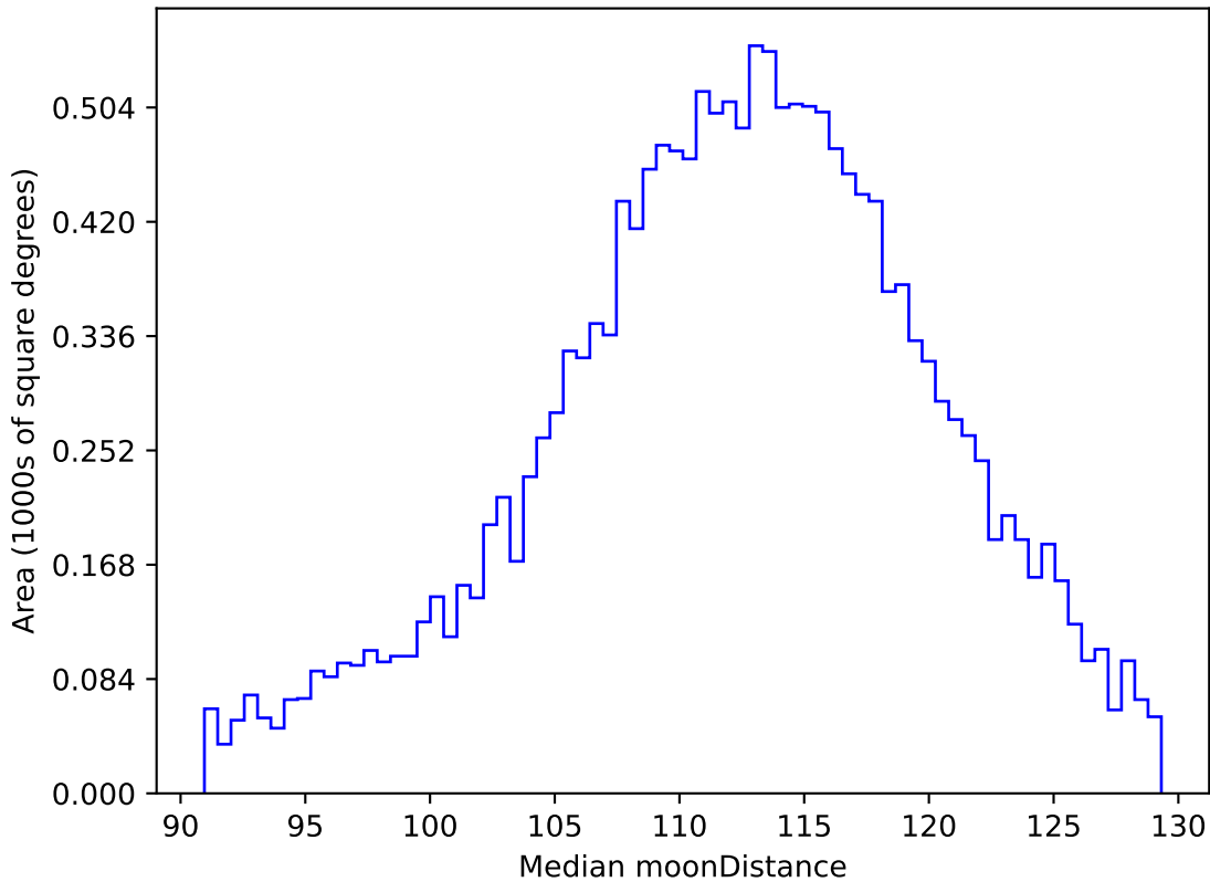
too_elab_r16_d2_giz_v3.4_10yrs WFD r band: Median moonDistance
