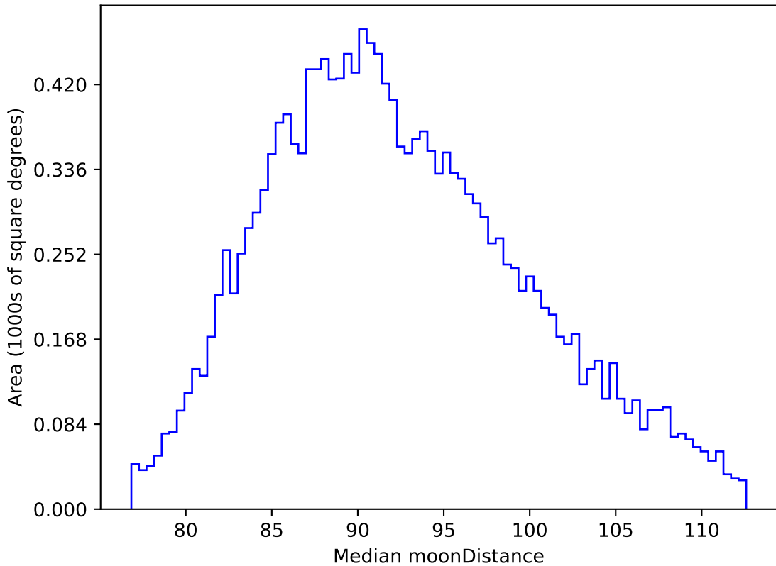
too_elab_r16_d2_giz_v3.4_10yrs WFD i band: Median moonDistance
