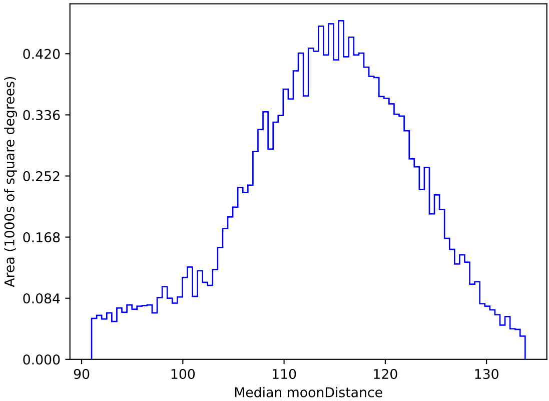
too_elab_r16_d2_giz_v3.4_10yrs WFD g band: Median moonDistance
