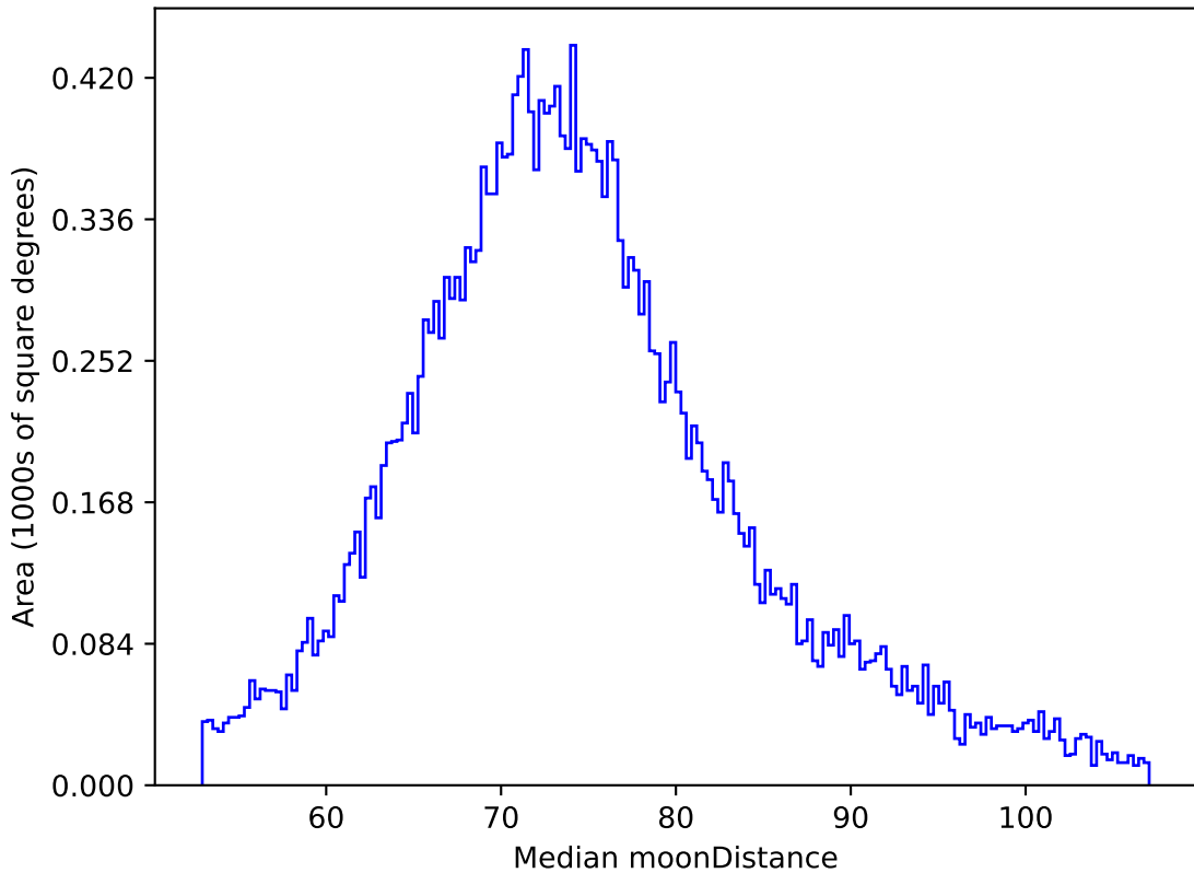
too_elab_r16_d2_giz_v3.4_10yrs All sky z band: Median moonDistance
