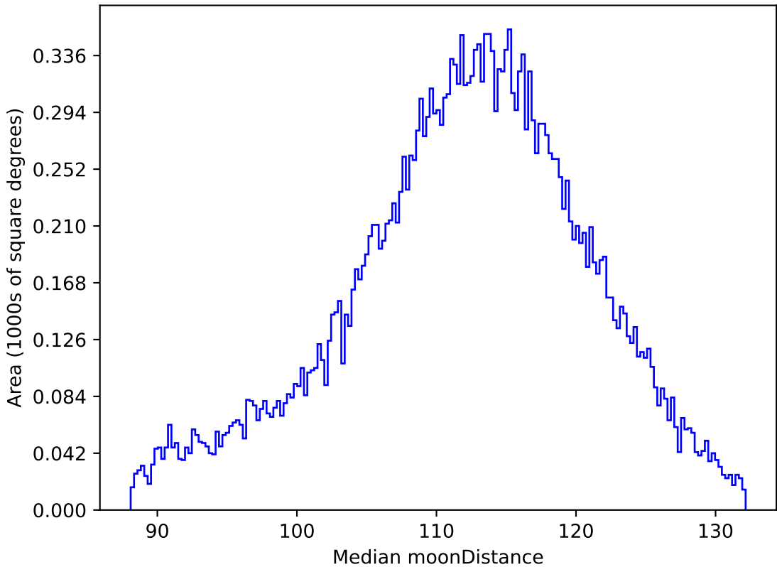
too_elab_r16_d2_giz_v3.4_10yrs All sky r band: Median moonDistance
