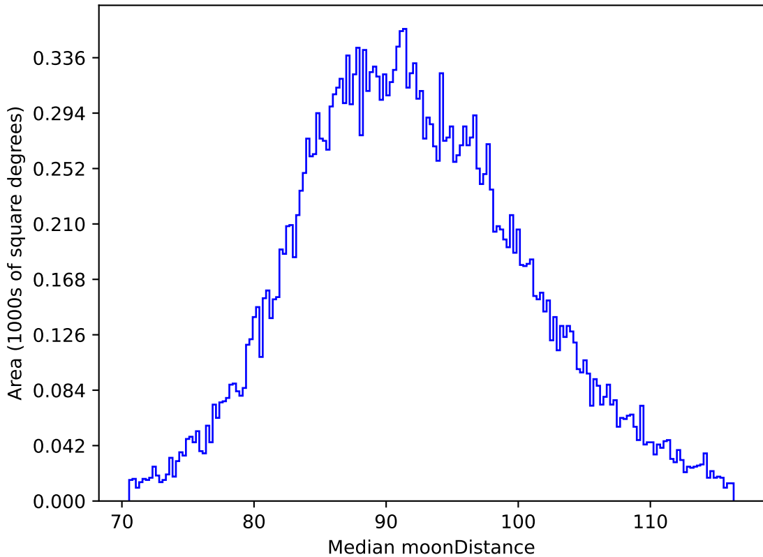
too_elab_r16_d2_giz_v3.4_10yrs All sky i band: Median moonDistance
