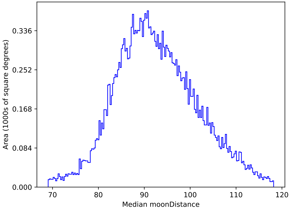
too_elab_r16_d2_giz_v3.4_10yrs All sky i band: Median moonDistance
