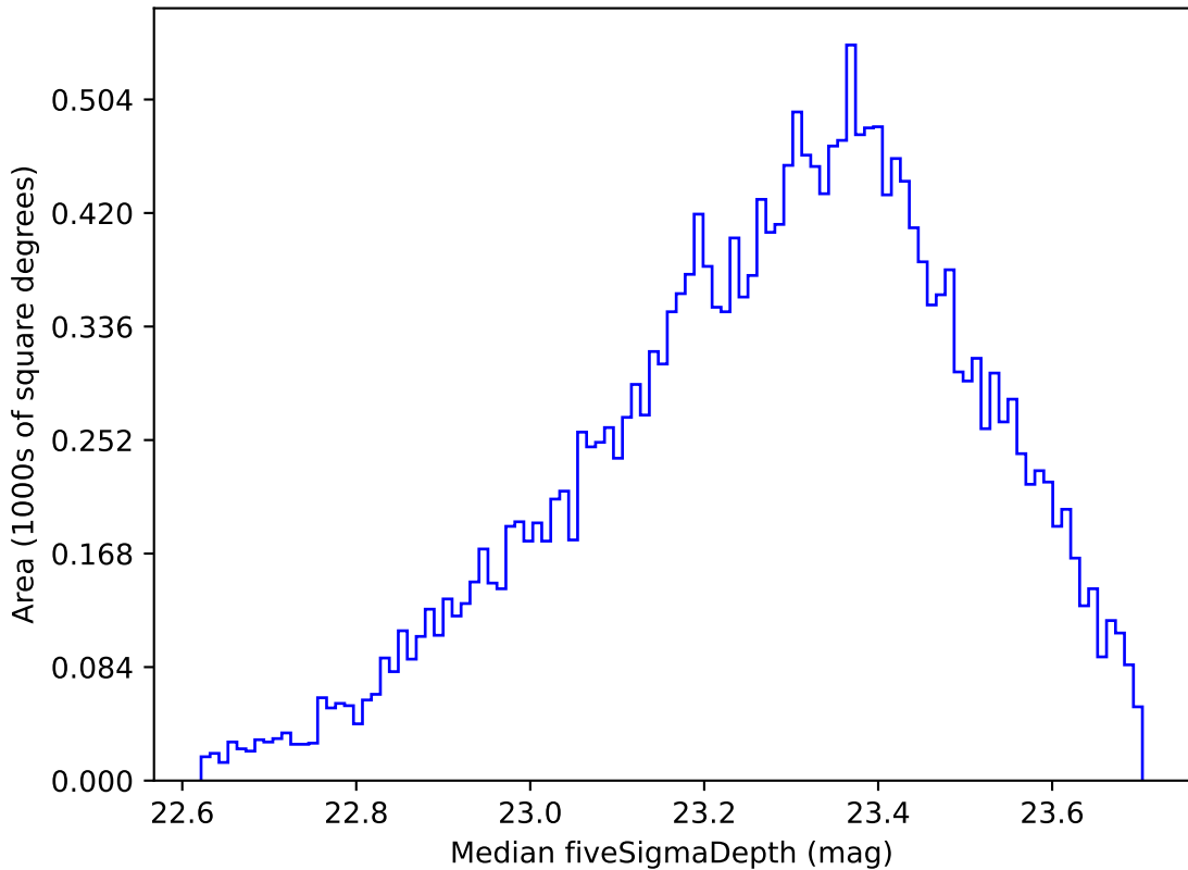
too_elab_r16_d2_giz_v3.4_10yrs Yr 1 u band: Median fiveSigmaDepth
